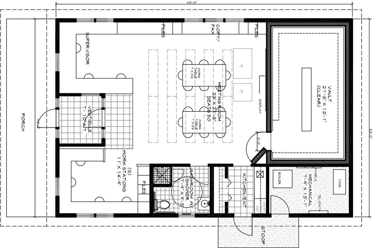
PROPOSED FLOOR PLAN SCALE: 1/8" = 1'-0"
